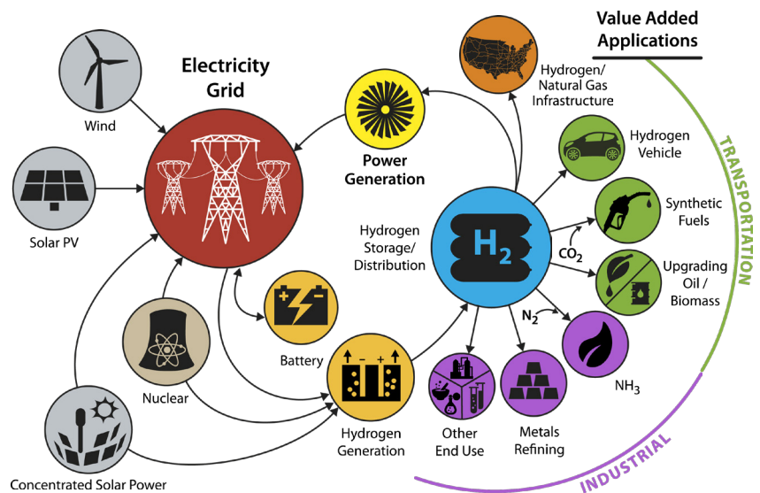
Figure 1. The Clean Energy Cycle: Hydrogen Technology's Central Role in Clean, Sustainable Energy. Courtesy of LNL and NREL
